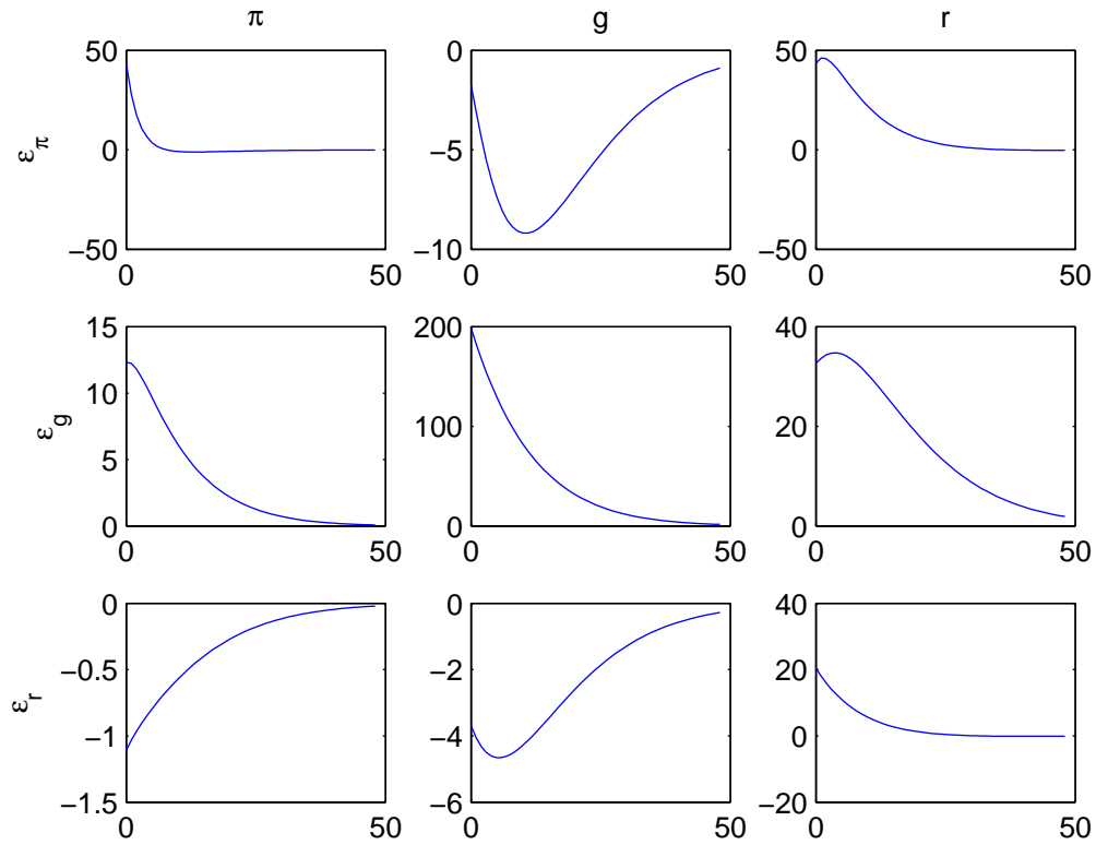
Figure 2: Impulse Responses of Macroeconomic Variables to Structural Shocks
