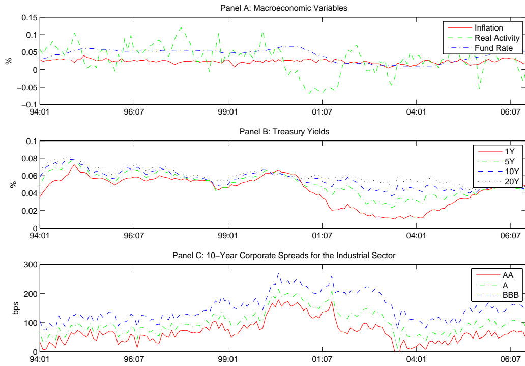
Figure 1: Macro Variables, Treasury Yields and Corporate Spreads
