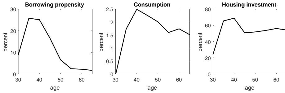
Figure 7: Differential responses to a permanent mortgage rate reduction
